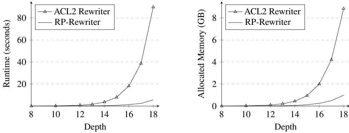
Figure 1: Performance comparison of ACL2's built-in rewriter and RP-Rewriter on a conjecture with a term tree of 4vec-bitand and logapp functions only using the rewrite rules from Example ??.
